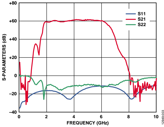
Figure 3. S-Parameters vs. Frequency at 25°C
