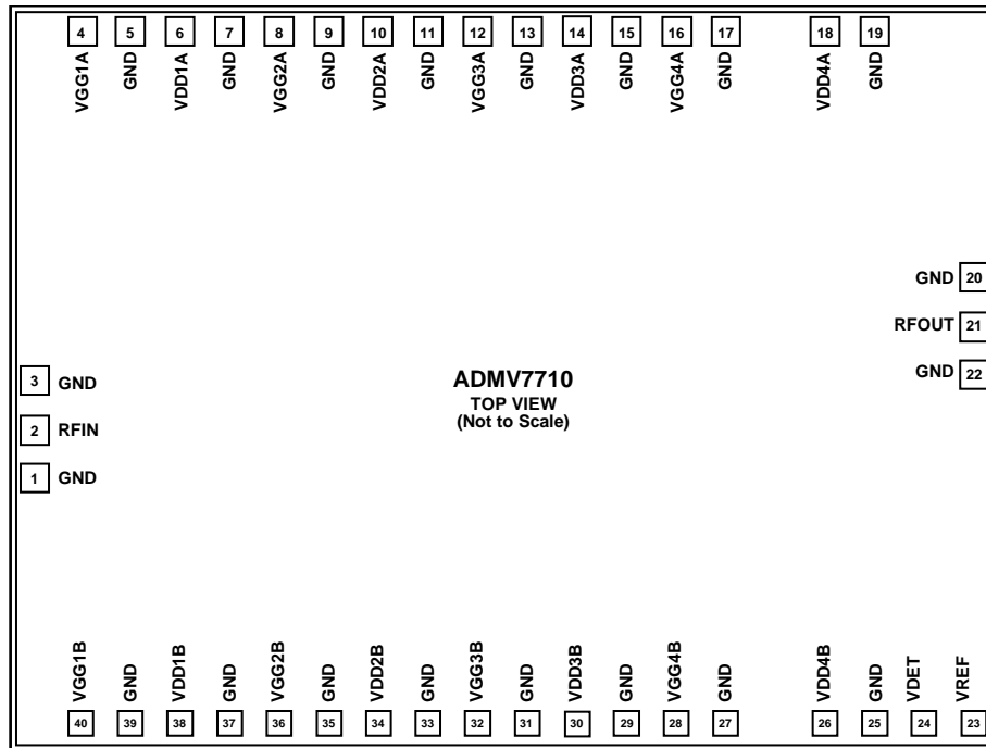
Figure 2. Pad Configuration
