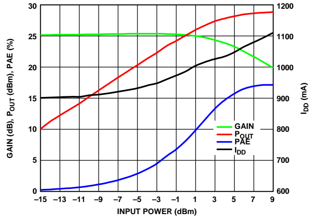
Figure 36. Gain, P_{OUT} , PAE, and I_{DD} vs. Input Power, RF = 76 GHz, I_{DD} = 900 mA
