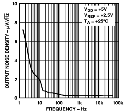
Figure 12. Output Noise Density vs. Frequency
