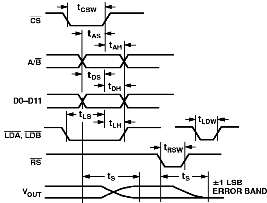
Figure 2. Timing Diagram
