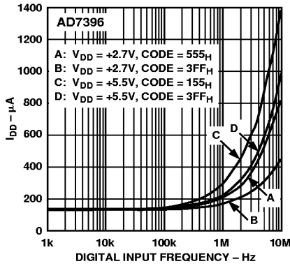
Figure 22. I_{DD} vs. Digital Input Frequency
