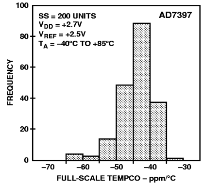
Figure 9. AD7397 Full-Scale Tempco Histogram
