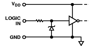
Figure 28. Equivalent Digital Input ESD Protection
