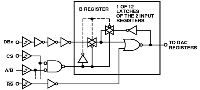
Figure 3. Digital Control Logic
