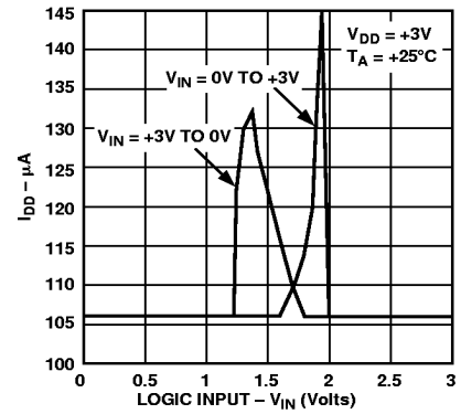
Figure 15. I_{DD} vs. Logic Input Voltage
