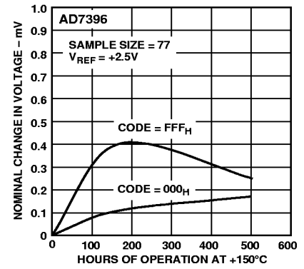
Figure 24. Long-Term Drift Accelerated by Burn-In
