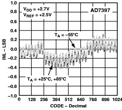
Figure 5. AD7397 INL vs. Code and Temperature
