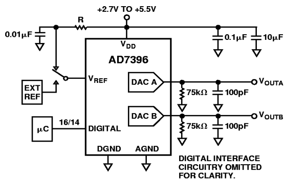
Figure 29. Unipolar Output Operation
