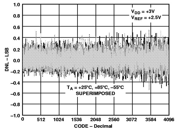
Figure 1. DNL vs. Digital Code at Temperature
