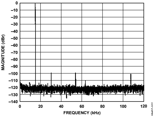
Figure 22. Wideband Plot, 15 kHz Input, 8x Interpolation, SR 48 kHz
