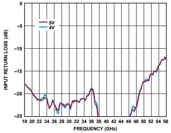
Figure 15. Input Return Loss vs. Frequency for Various Supply Voltages, I_{DQ} = 1500\text{ mA}
