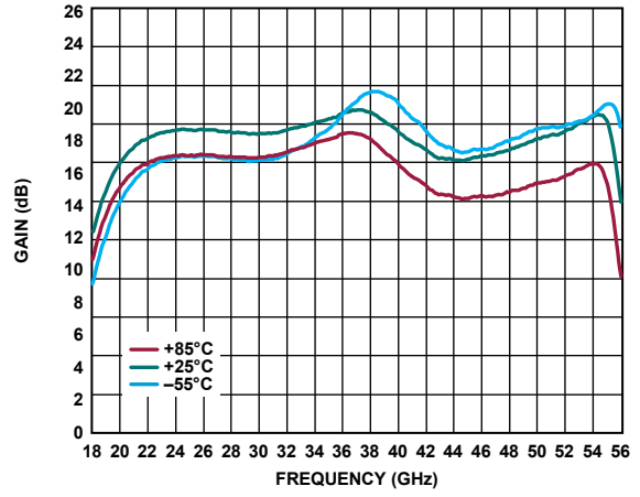
Figure 13. Gain vs. Frequency for Various Temperatures, V_{DD} = 5\text{ V} , I_{DQ} = 1500\text{ mA}
