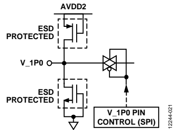
Figure 62. V_1P0 Input
