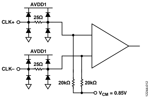
Figure 53. Clock Inputs
