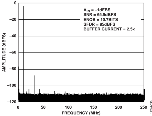
Figure 29. Single-Tone FFT with Input Frequency ( f_{IN} ) = 10.3 MHz
