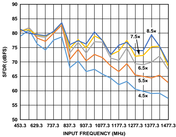
Figure 68. Buffer Current Sweeps, AD9234-1000; SFDR vs. Input Frequency ( I_{BUFF} ); 500 \text{ MHz} < f_{IN} < 1500 MHz
