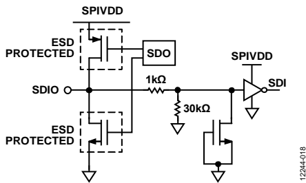
Figure 59. SDIO Input
