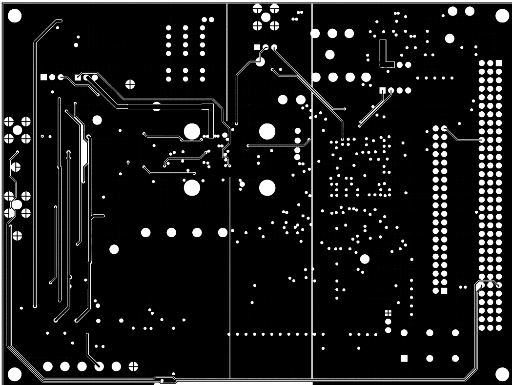
Figure 8. Shield Layer
