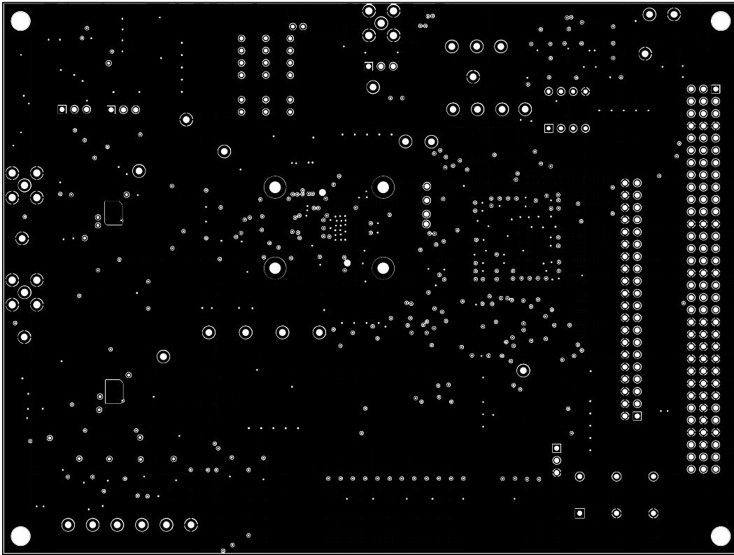
Figure 7. Ground Layer
