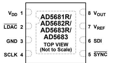
Figure 6. Pin Configuration, 8-Lead LFCSP, \overline{\text{LDAC}} Option
