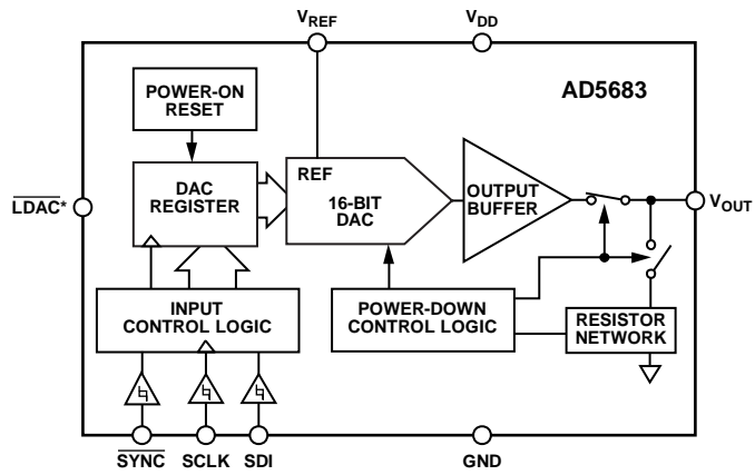
Figure 3. AD5683 LFCSP
