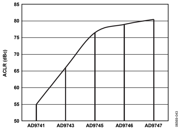
Figure 20. ACLR vs. Bit Resolution, Single Carrier WCDMA, 245.76 MSPS, f_{CARRIER} = 61.44 MHz
