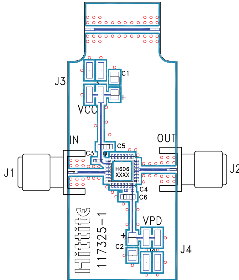
Figure 17. Evaluation PCB
