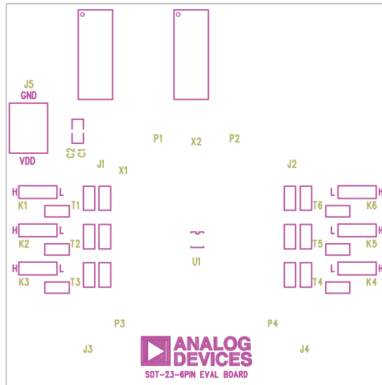
Figure 3. EVAL-6SOT23EBZ Silkscreen
