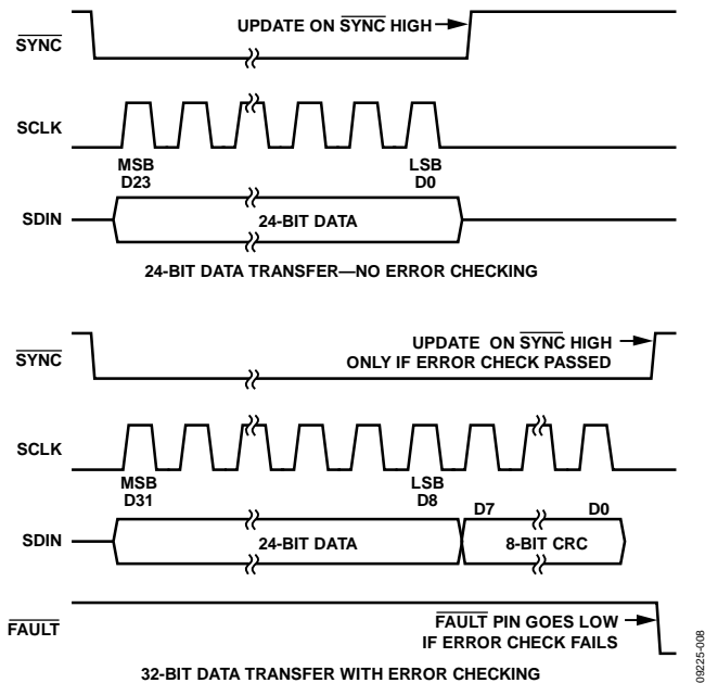
Figure 55. PEC Timing
