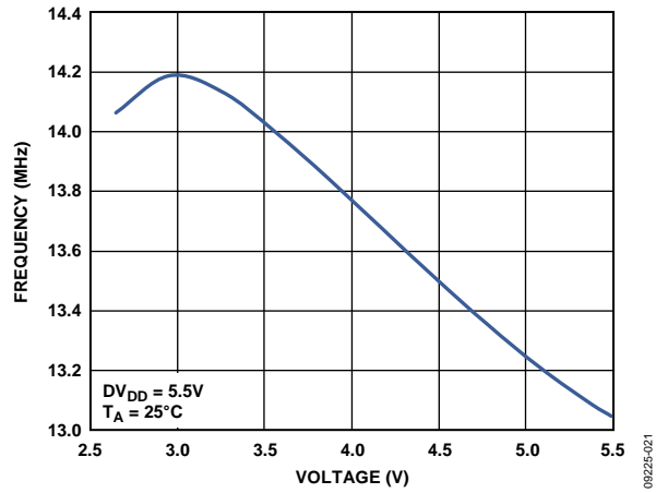
Figure 48. Internal Oscillator Frequency vs. D V DD Supply Voltage
