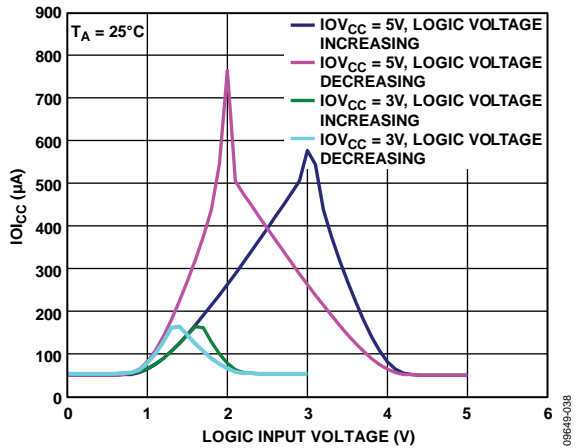
Figure 37. I OC vs. Logic Input Voltage
