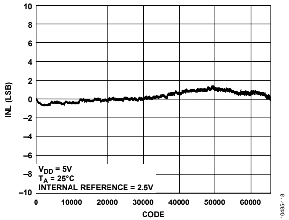
Figure 15. AD5686R INL
