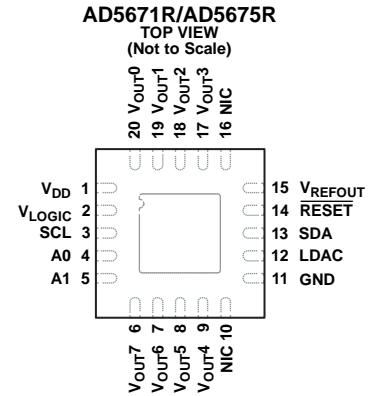
Figure 5. LFCSF Pin Configuration
