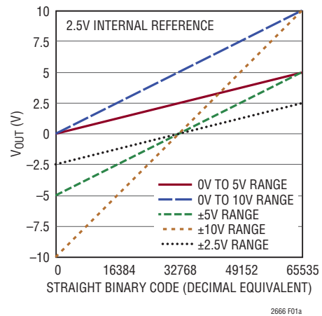
Figure 2a. LTC2666-16 Transfer Function
