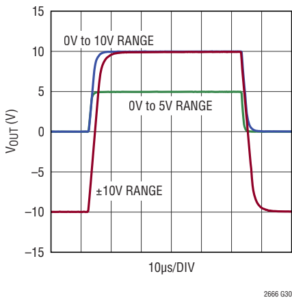
Large Signal Response
