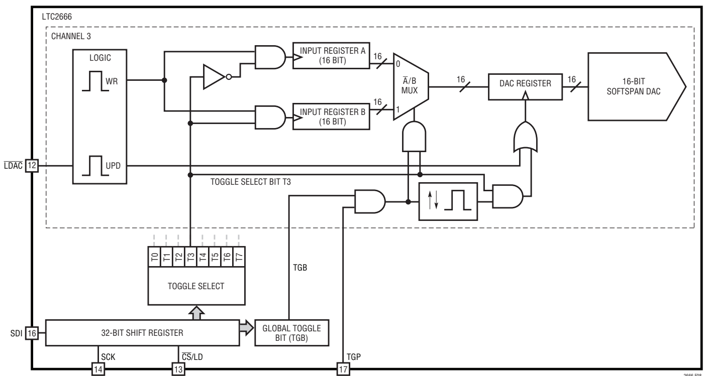
Figure 8. Simplified Toggle Block Diagram. Conceptual Only, Actual Circuit May Differ
