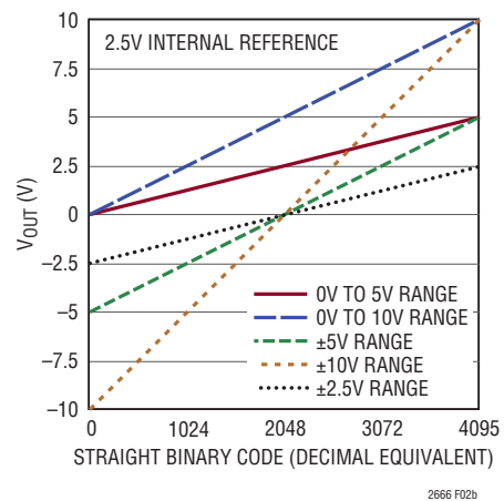
Figure 2b. LTC2666-12 Transfer Function
