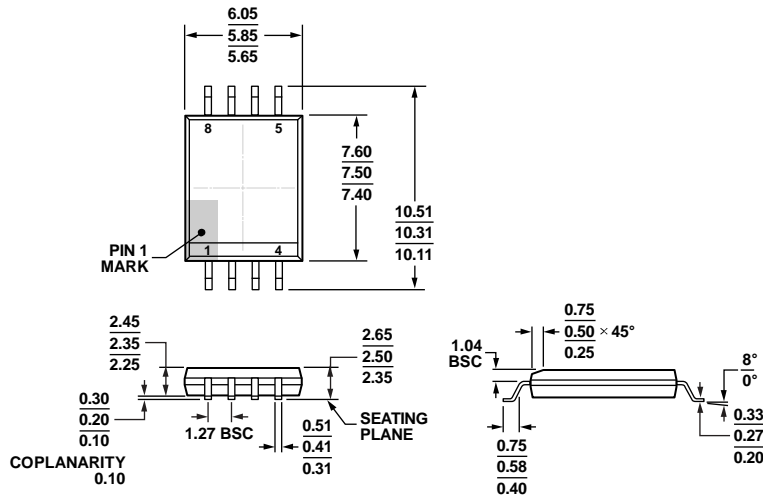
Figure 40. 8-Lead Standard Small Outline Package, with Increased Creepage [SOIC_IC] Wide Body (RI-8-1) Dimensions shown in millimeters
