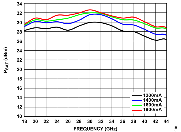
Figure 50. P SAT vs. Frequency for Various I DD , V DD = 5 V, Data Measured with Constant I DD
