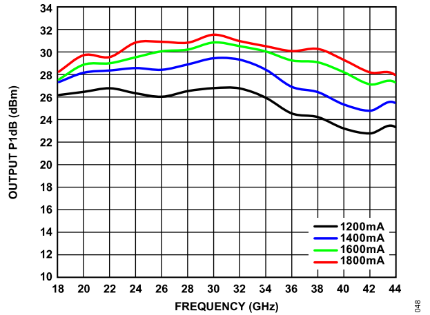
Figure 49. Output P1dB vs. Frequency for Various I DD , V DD = 5 V, Data Measured with Constant I DD
