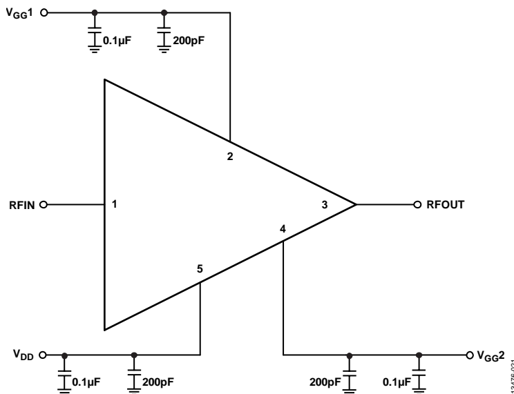
Figure 22. Applications Circuit
