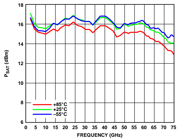
Figure 13. PSAT vs. Frequency at Various Temperatures
