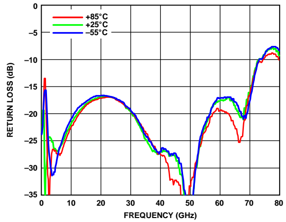
Figure 12. Output Return Loss at Various Temperatures
