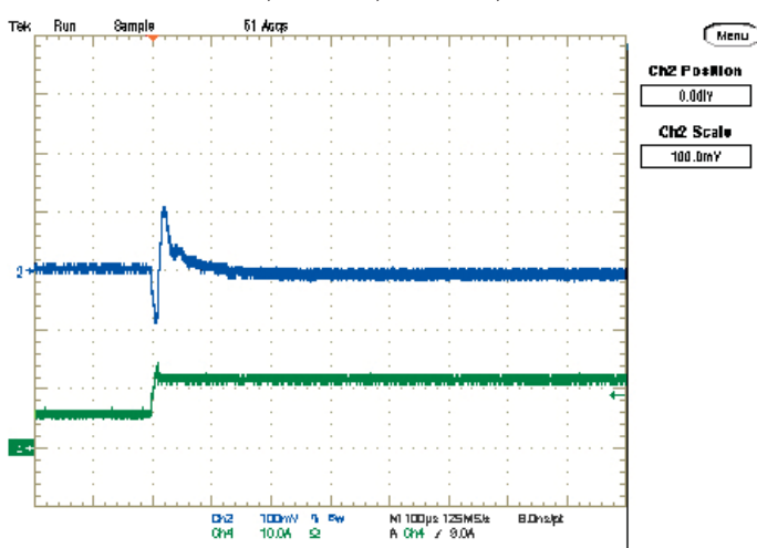
Step Load Transient Response (Vin=11V, Vout=1.2V, Cload=188µF, Iout=6A to 12A) Trace 2=Vout, 100 mV/div, Trace 4=Iout, 10A/div.
