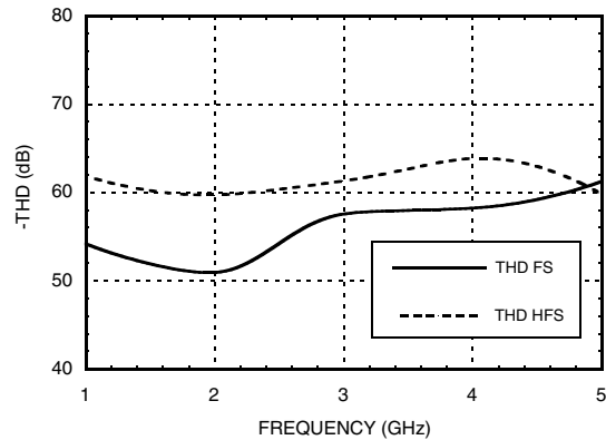
Hold-Mode THD vs. Frequency & Input Power @ f_{clk} = 4 \text{ GHz} @ 0 \text{ dBm}
