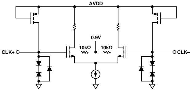
Figure 56. Equivalent Clock Input Circuit
