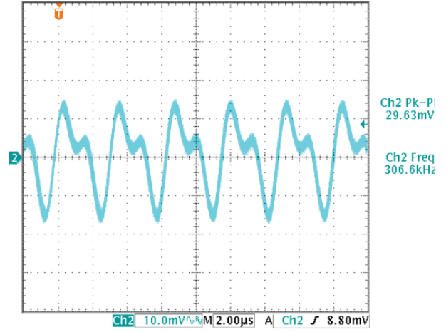
Output Ripple and Noise (Vin=5V, Iout=5A, Vout=1V, Cout= 1uF || 10uF, Ta=+25°C)
