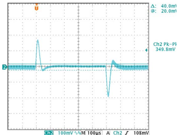
Step Load Transient Response (Vin=5V, Vout=1V, Iout=50-100-50% load (2.5A/us), Ta=+25°C)
