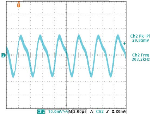
Output Ripple and Noise (Vin=5V, Iout=5A, Vout=1.8V, Cout= 1uF || 10uF, Ta=+25°C)
