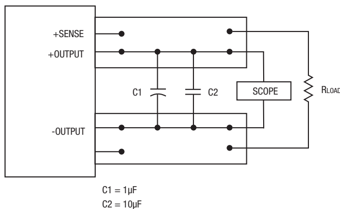
Figure 3. Measuring Output Ripple and Noise (PARD)
