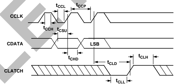
Figure 22. Serial Control Port Timing
