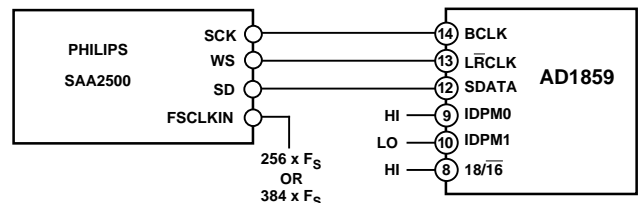
Figure 14. Interface to SAA2500
