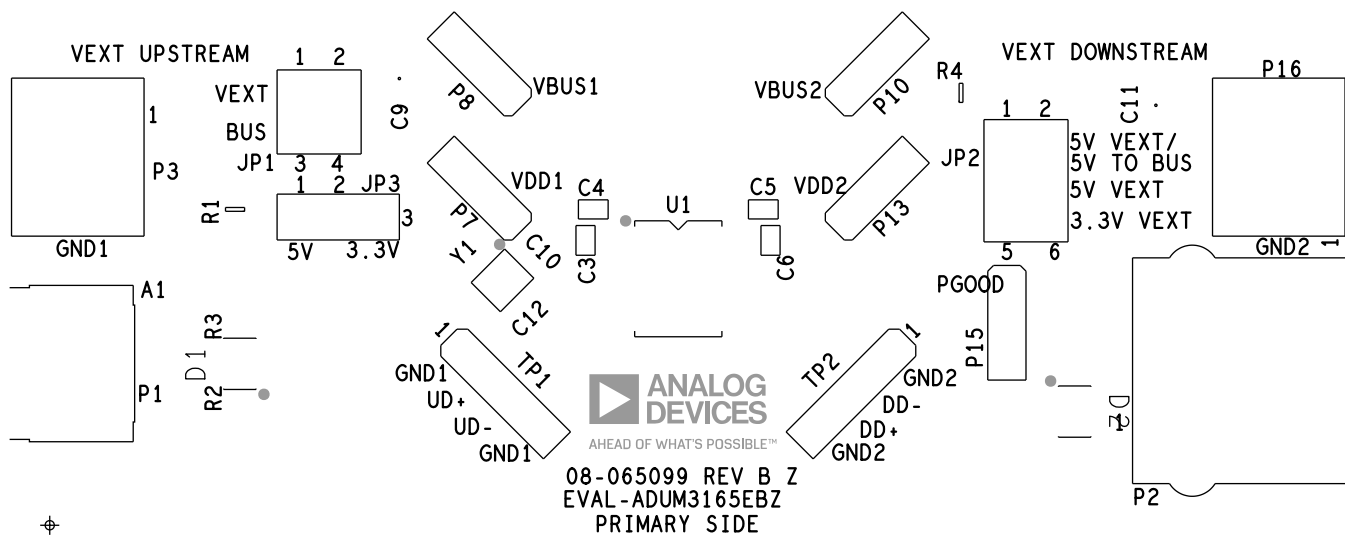
Figure 9. EVAL-ADuM3165EBZ Silkscreen
