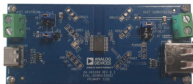
Figure 1. EVAL-ADuM3165EBZ Photograph
