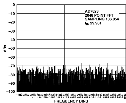
Figure 3. AD7823 SNR
