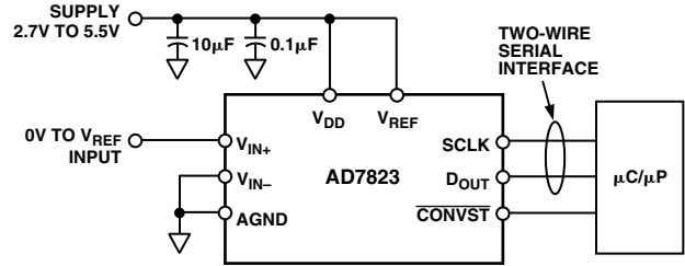
Figure 6. Typical Connection Diagram
