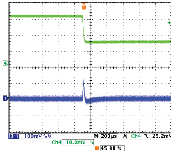
Step Load Transient Response (Vin=5V, Vout=2.5V, Cload=0, Iout=16A to 8A) Trace 1=Vout, 100 mV/div. Trace 4=Iout, 5A/div.
