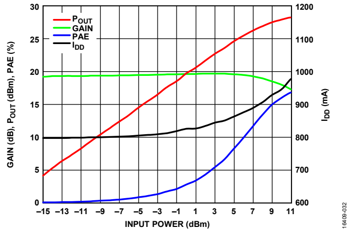
Figure 32. Gain, P_{OUT} , PAE, and I_{DD} vs. Input Power, RF = 83.5 GHz, I_{DD} = 800 mA
