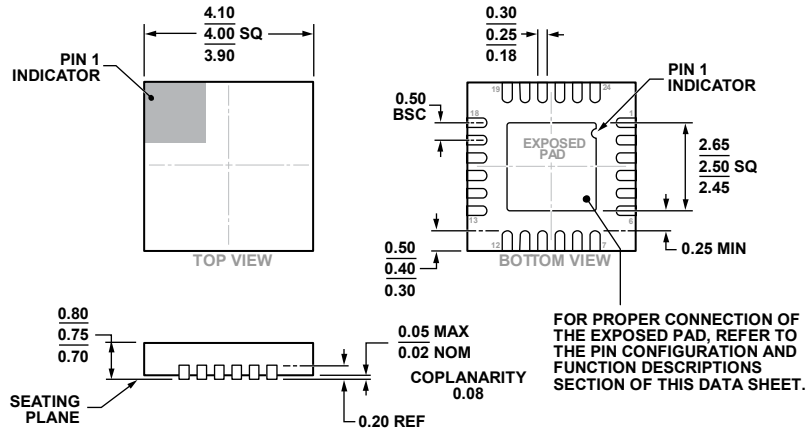
Figure 67. 24-Lead Lead Frame Chip Scale Package [LFCSQ_WQ] 4 mm × 4 mm Body, Very Very Thin Quad (CP-24-7) Dimensions shown in millimeters
