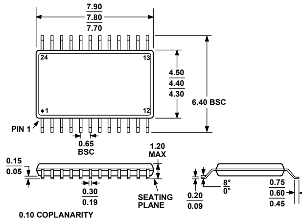
Figure 68. 24-Lead Thin Shrink Small Outline Package [TSSOP] (RU-24) Dimensions shown in millimeters
