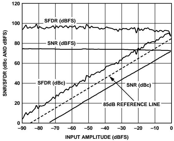
Figure 28. AD9640-150 Single-Tone SNR/SFDR vs. Input Amplitude ( A_{IN} ) with f_{IN} = 2.3 MHz
