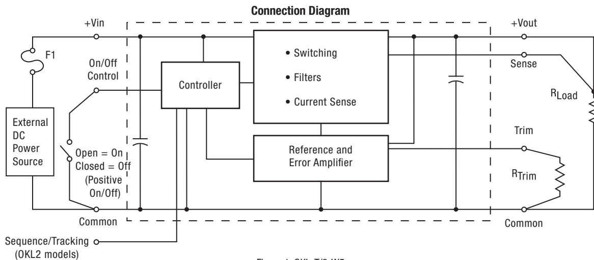
Figure 1. OKL-T/3-W5
