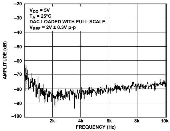
Figure 48. Total Harmonic Distortion
