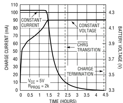
Complete Charge Cycle (180mAh Battery)
