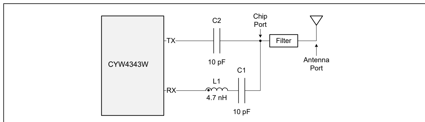
Figure 35. RF Port Location
