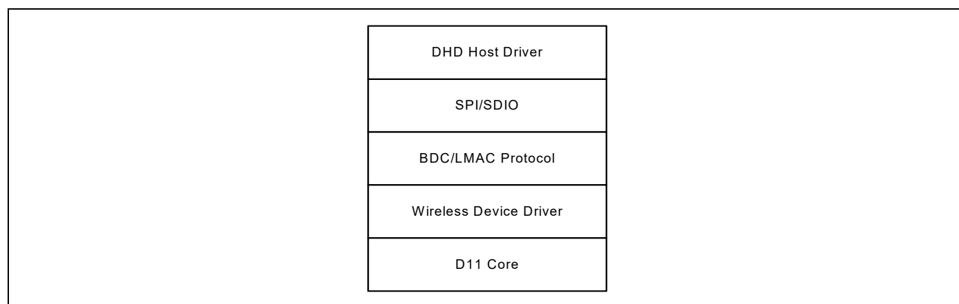
Figure 32. WLAN Software Architecture
