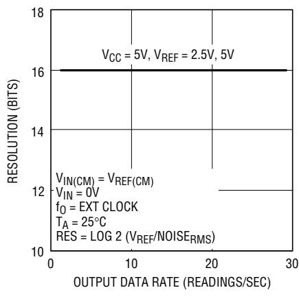
Figure 36. Resolution ( N_{RMS} \leq 1LSB ) vs Output Data Rate and Reference Voltage
