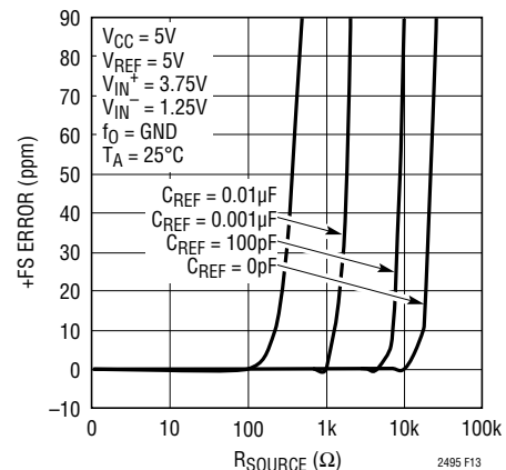
Figure 13. +FS Error vs R_{\text{SOURCE}} at V_{\text{REF}} (Small C_{\text{REF}} )
