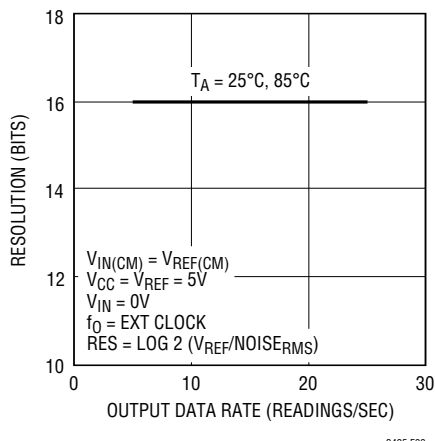
Figure 33. Resolution ( N_{RMS} \leq 1LSB ) vs Output Data Rate and Temperature
