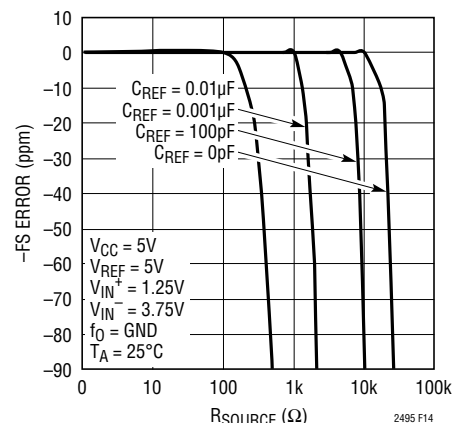
Figure 14. -FS Error vs R_{\text{SOURCE}} at V_{\text{REF}} (Small C_{\text{REF}} )
