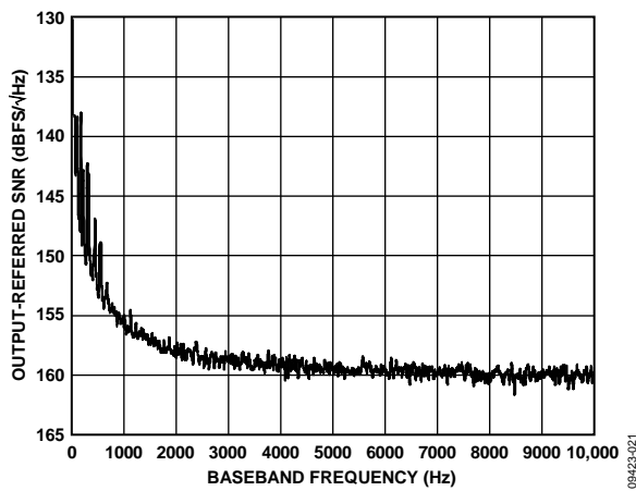
Figure 24. Output-Referred SNR vs. Baseband Frequency
