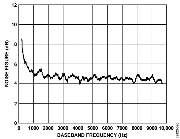
Figure 23. Noise Figure vs. Baseband Frequency
