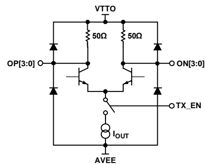
Figure 26. High Speed Output Simplified Schematic
