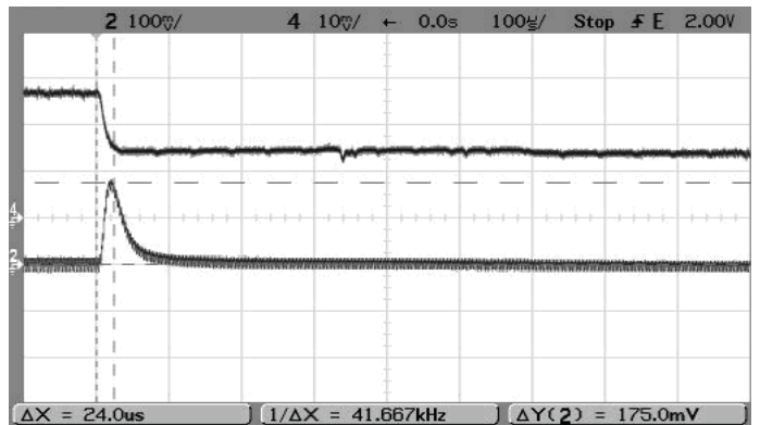
Step Load Transient Response (Vin=5V, Vout=3.3V, Cload=0, Iout=5A to 2.5A) Trace 2=Vout, 100 mV/div. Trace 4=Iout, 2A/div.
