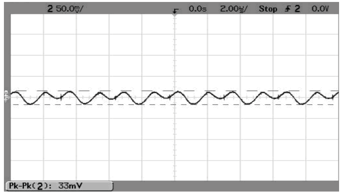
Output Ripple and Noise (Vin=5V, Vout=3.3V, Iout=5A, Cload=0, ScopeBW=100MHz)
