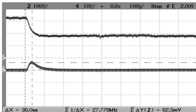
Step Load Transient Response (Vin=5V, Vout=2.5V, Load=0, Iout=3A to 1.5A) Trace 2=Vout, 100 mV/div. Trace 4=Iout, 1A/div.
