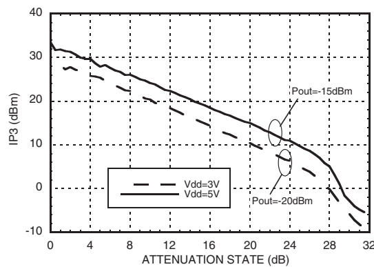
Output IP3 vs. Attenuation @ 900 MHz [1]
