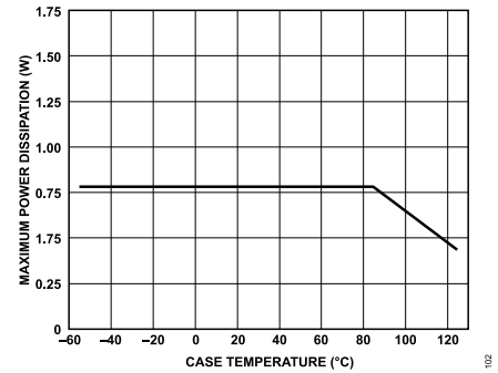
Figure 2. Maximum Power Dissipation vs. Case Temperature
