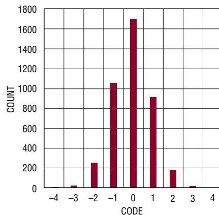
Figure 5. LTC1856 Histogram for 4096 Conversions
