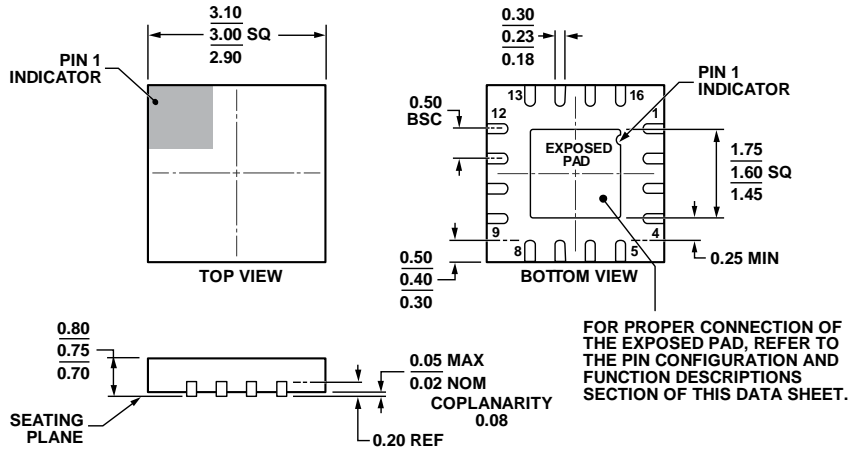
COMPLIANT TO JEDEC STANDARDS MO-220-WEED-6. Figure 53. 16-Lead Lead Frame Chip Scale Package [LFCSP_WQ] 3 mm x 3 mm Body, Very Very Thin Quad (CP-16-22) Dimensions shown in millimeters
