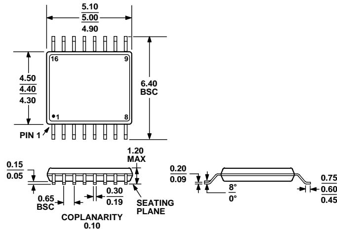
COMPLIANT TO JEDEC STANDARDS MO-153-AB Figure 54. 16-Lead Thin Shrink Small Outline Package [TSSOP] (RU-16) Dimensions shown in millimeters
