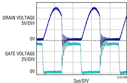
Figure 6. Voltage on the Drain and Gate of NMOS, M1, when f_{TX-TANK} = f_{DRIVE}
