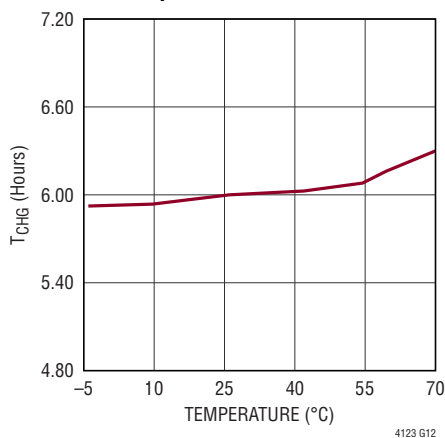
Charge Termination Period vs Temperature
