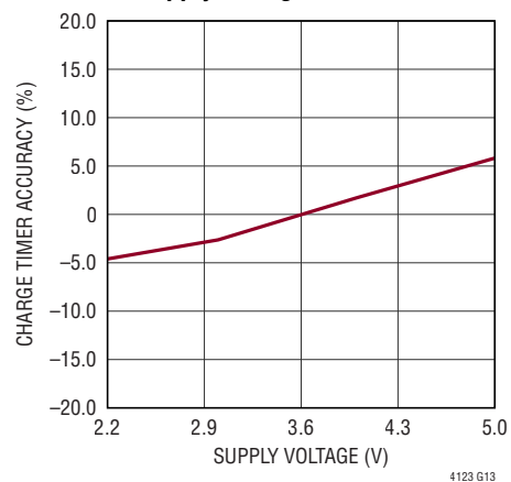
Charge Timer Accuracy vs Supply Voltage
