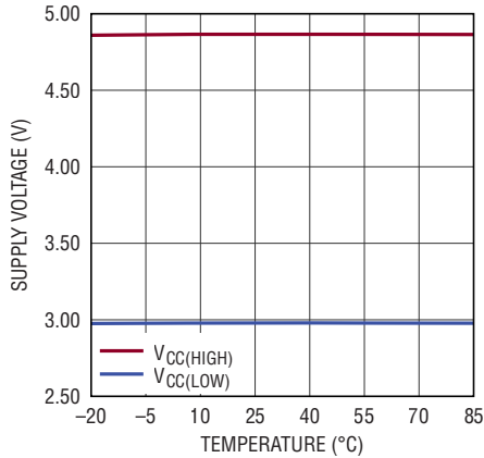
V_{CC} High and Low Thresholds vs Temperature
