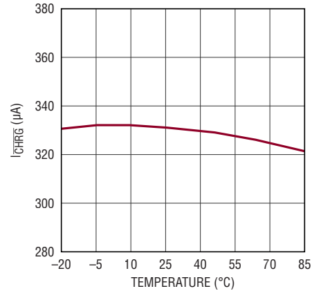
CHRG Pull-Down Current vs Temperature
