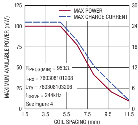
Maximum Available Wireless Power vs Coil Spacing
