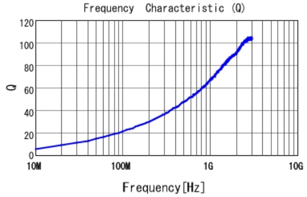
LQW15AN6N8H0Z Q
