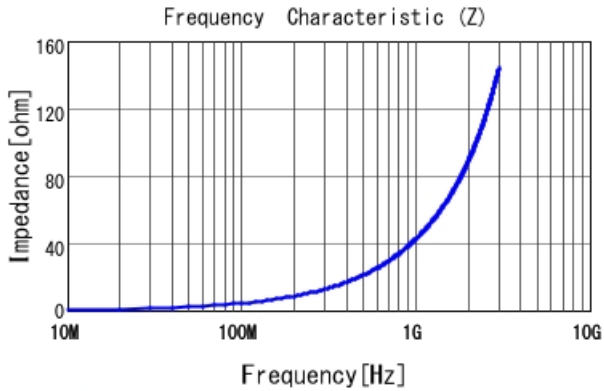
LQW15AN6N8H0Z |Z|
