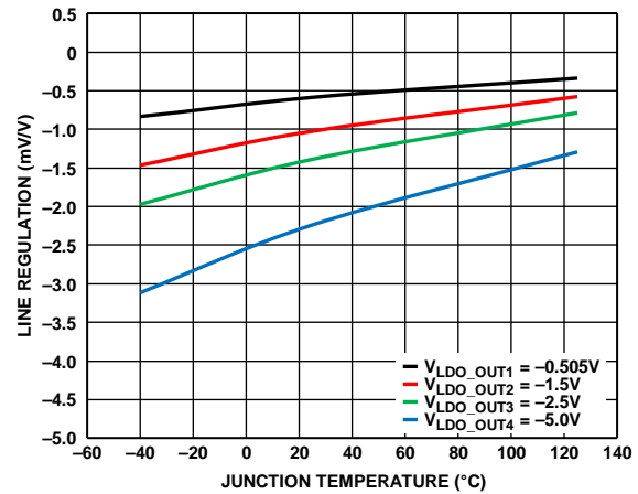
Figure 5. LDO Line Regulation
