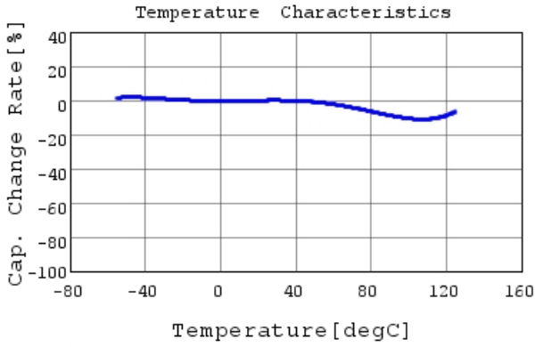
RDER72J102K2K1H03B C-Temp. capchange, DCOV,
