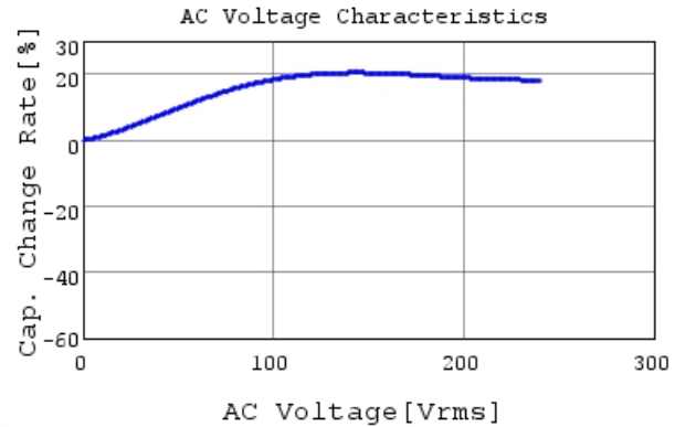
RDER72J102K2K1H03B C-AC Voltage capchange, I
