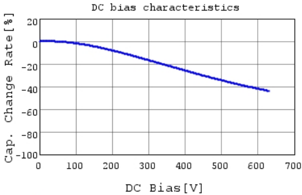
RDER72J102K2K1H03B C-DC bias capchange, 25.0
