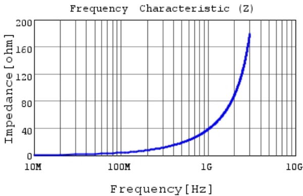
LQG15HZ6N2C02 |Z|
