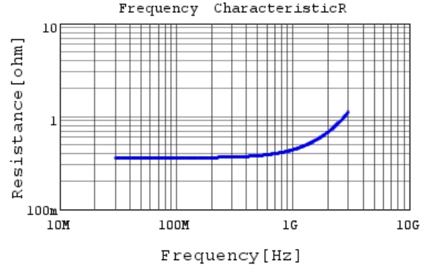
RDE5C2A100J0K1H03B R DC0V, 25degC
