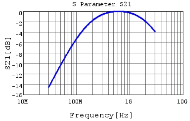
RDE5C2A100J0K1H03B S21 DCOV, 25degC
