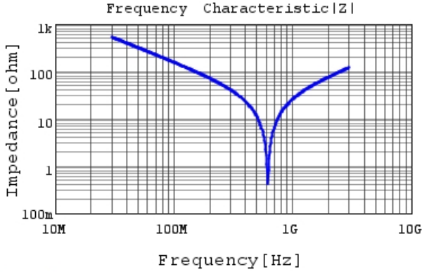
RDE5C2A100J0K1H03B |Z| DC0V, 25degC
