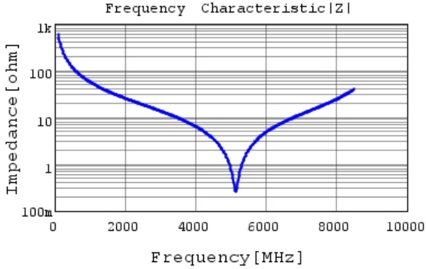
GCQ1555C1H2R7WB01 |Z| DC0V, 25degC
