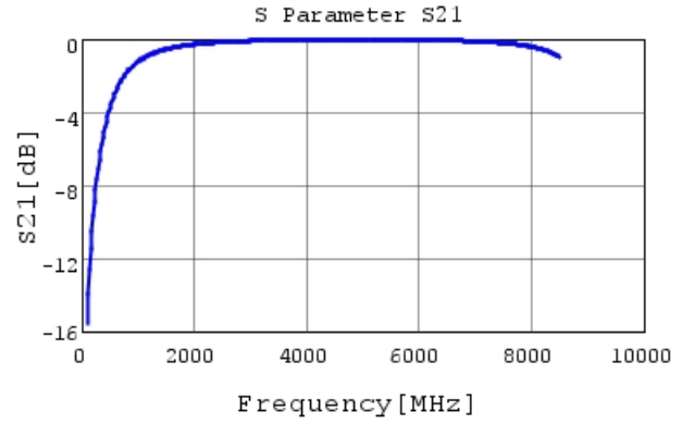
GCQ1555C1H2R7WB01 S21 DCOV, 25degC
