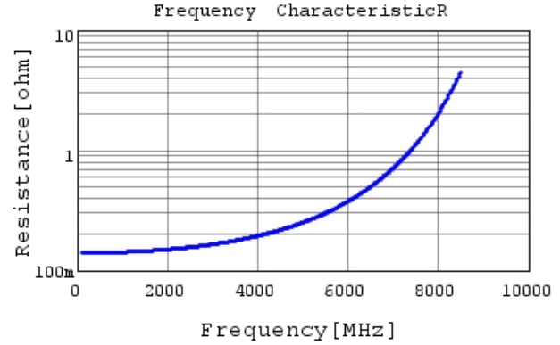
GCQ1555C1H2R7WB01 R DC0V, 25degC
