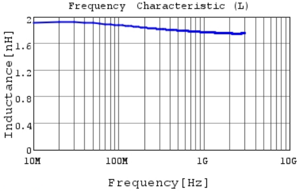
LQP02HQ1N8B02 L
