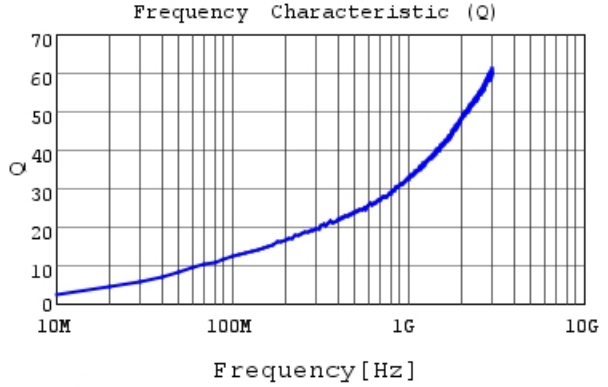
LQP02HQ1N8B02 Q
