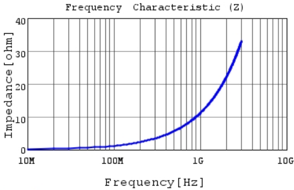
LQP02HQ1N8B02 |Z|
